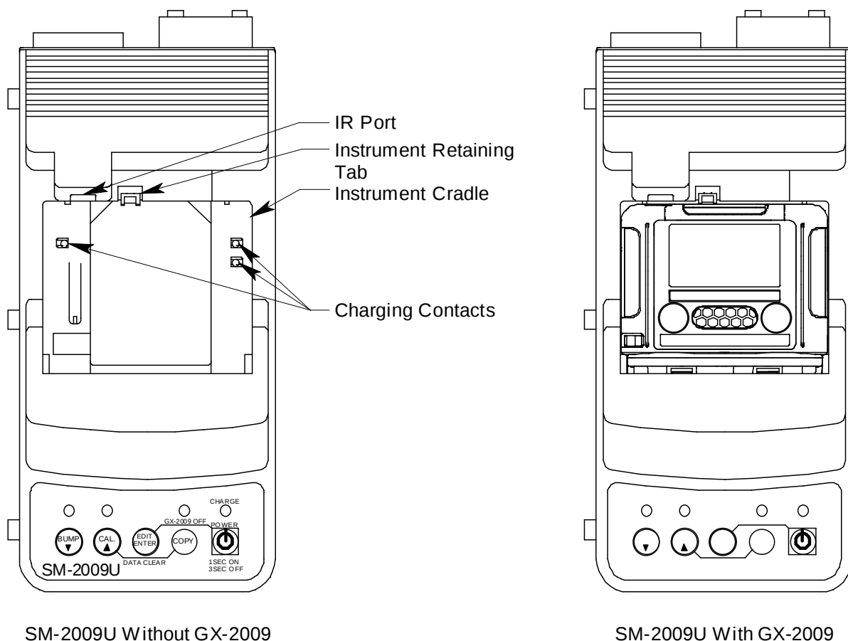
Figure 3: Instrument Cradle
