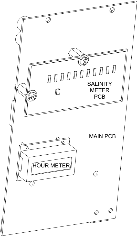
PCB MAIN ASSEMBLY PART NUMBER B596800012
