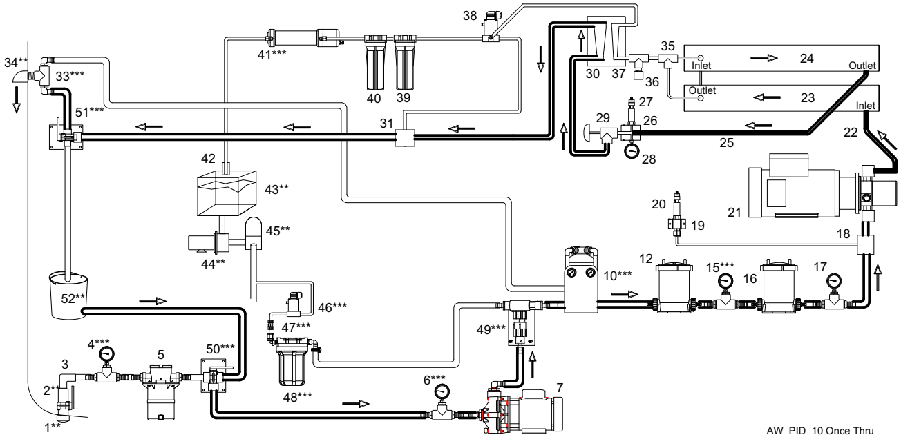
Aqua Whisper II Illustrated in a Once Through Configuration for Flushing the System with Fresh Water, and for discharging Cleaning or Storage Chemical
