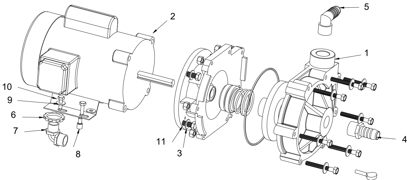
MAINTENANCE IMPELLER KIT 291211181PP
