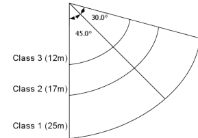
Vertical Field of View
