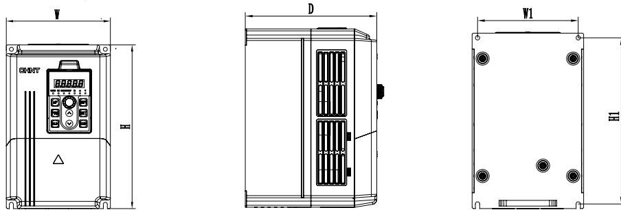
NVF2G-S-1.5/PS4 ~ NVF2G-S-11/PS4
