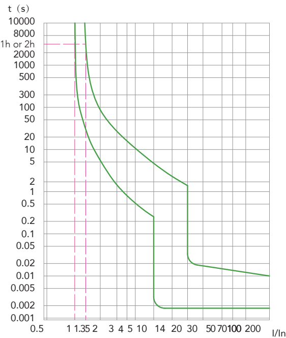
D Curve (B1H/B1N/B1NQ) (10~20 In)
