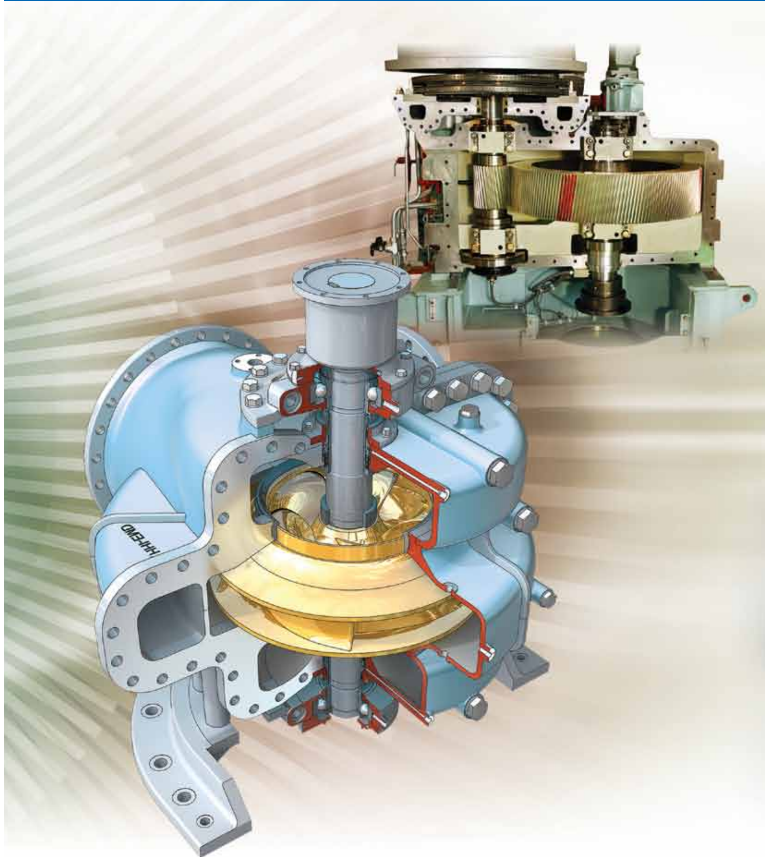
04_HYUNDAI CARGO OIL PUMPING SYSTEM
