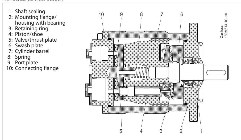
PAH 20/25/32 cross-section
