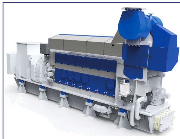
Figure 1: PTO on front end - external pump
