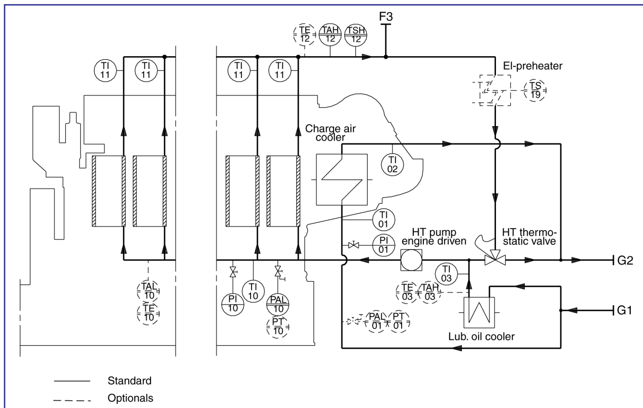
Figure 1: Diagram for internal cooling water system 1 (for guidance only, please see the plant specific engine diagram)
