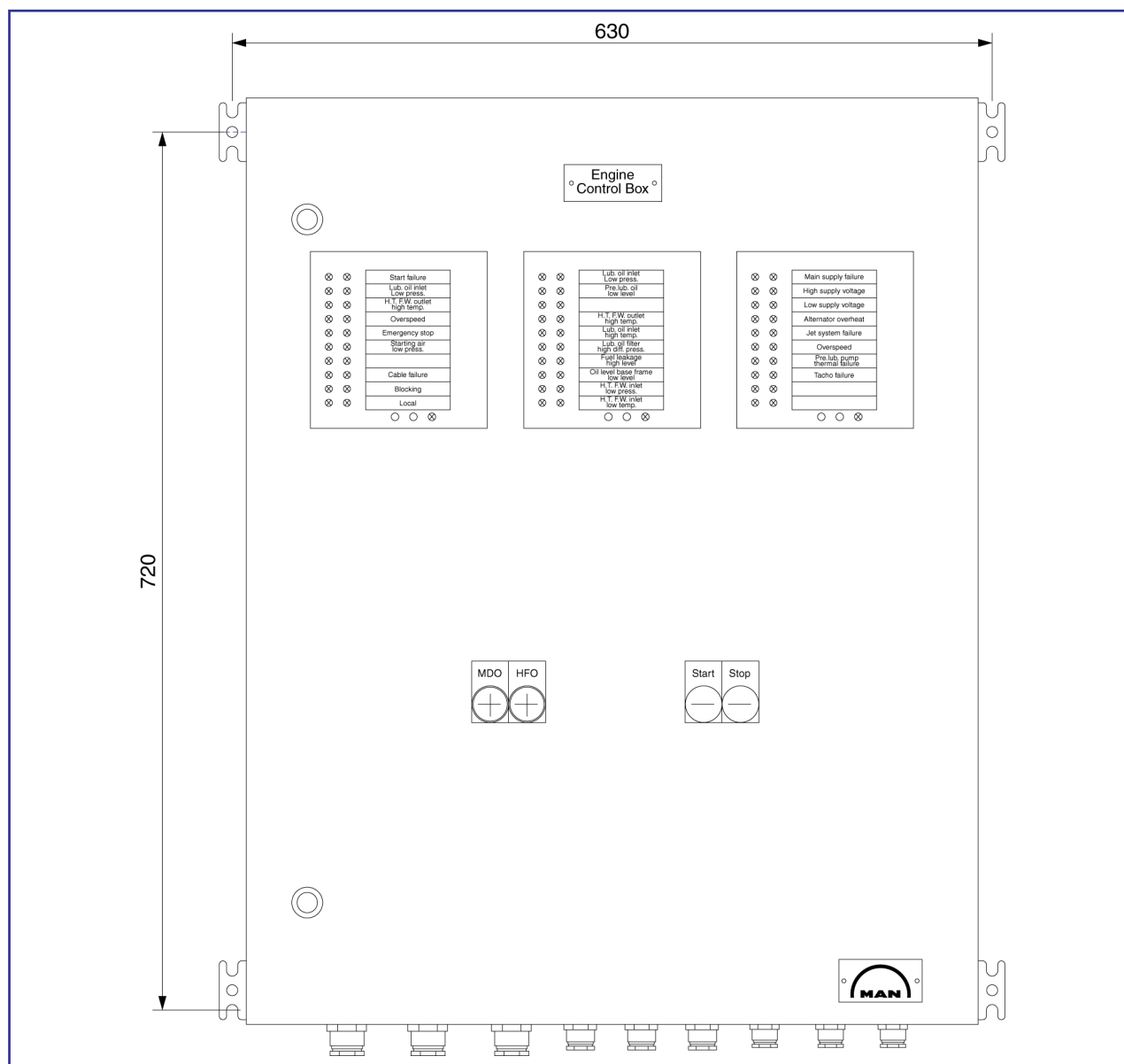
Figure 1: Engine control box.
