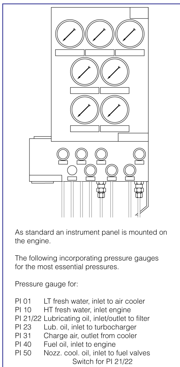
Figure 1: Lay-out of instrument panel.
