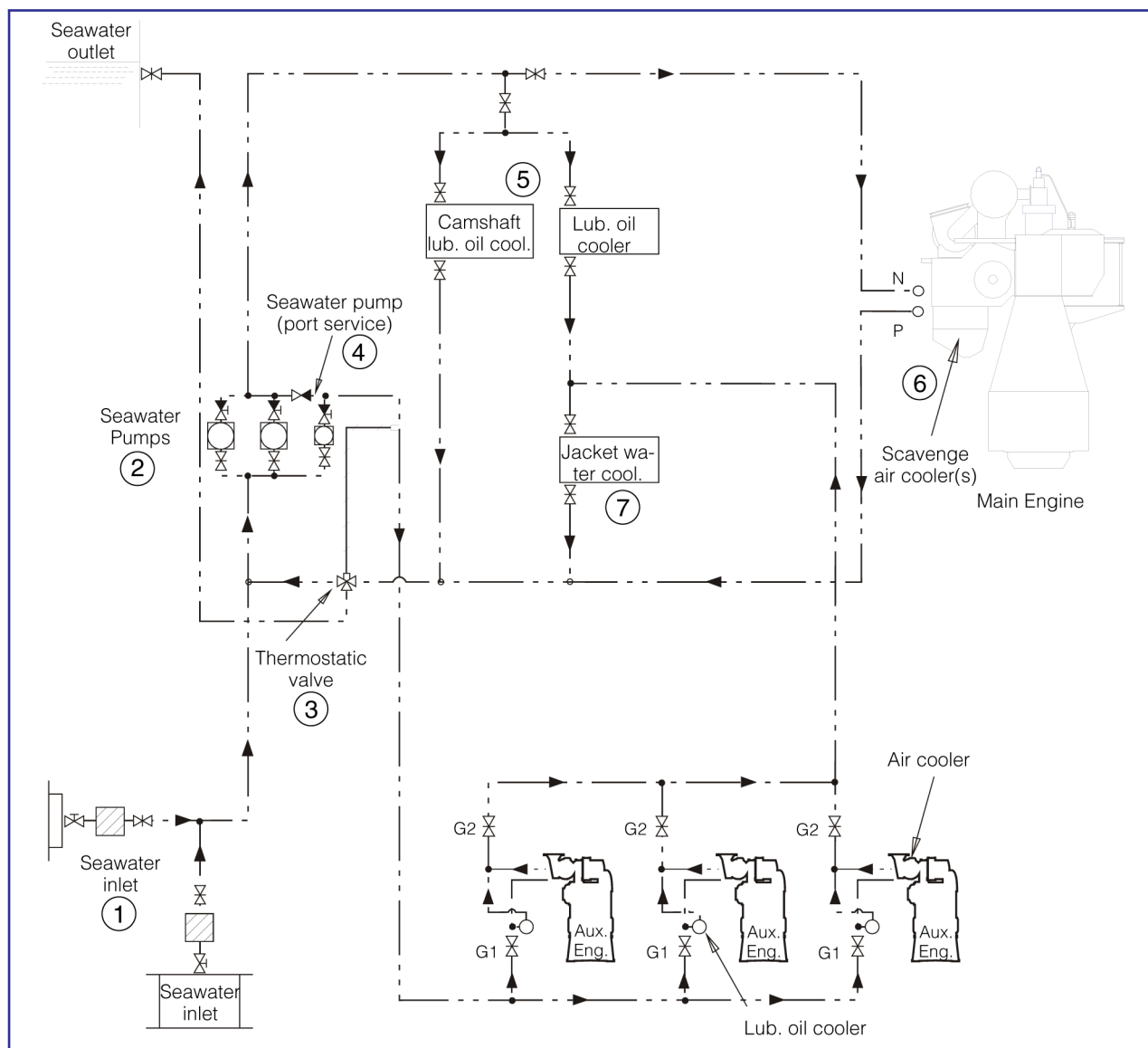
Figure 1: Sea water cooling system.
