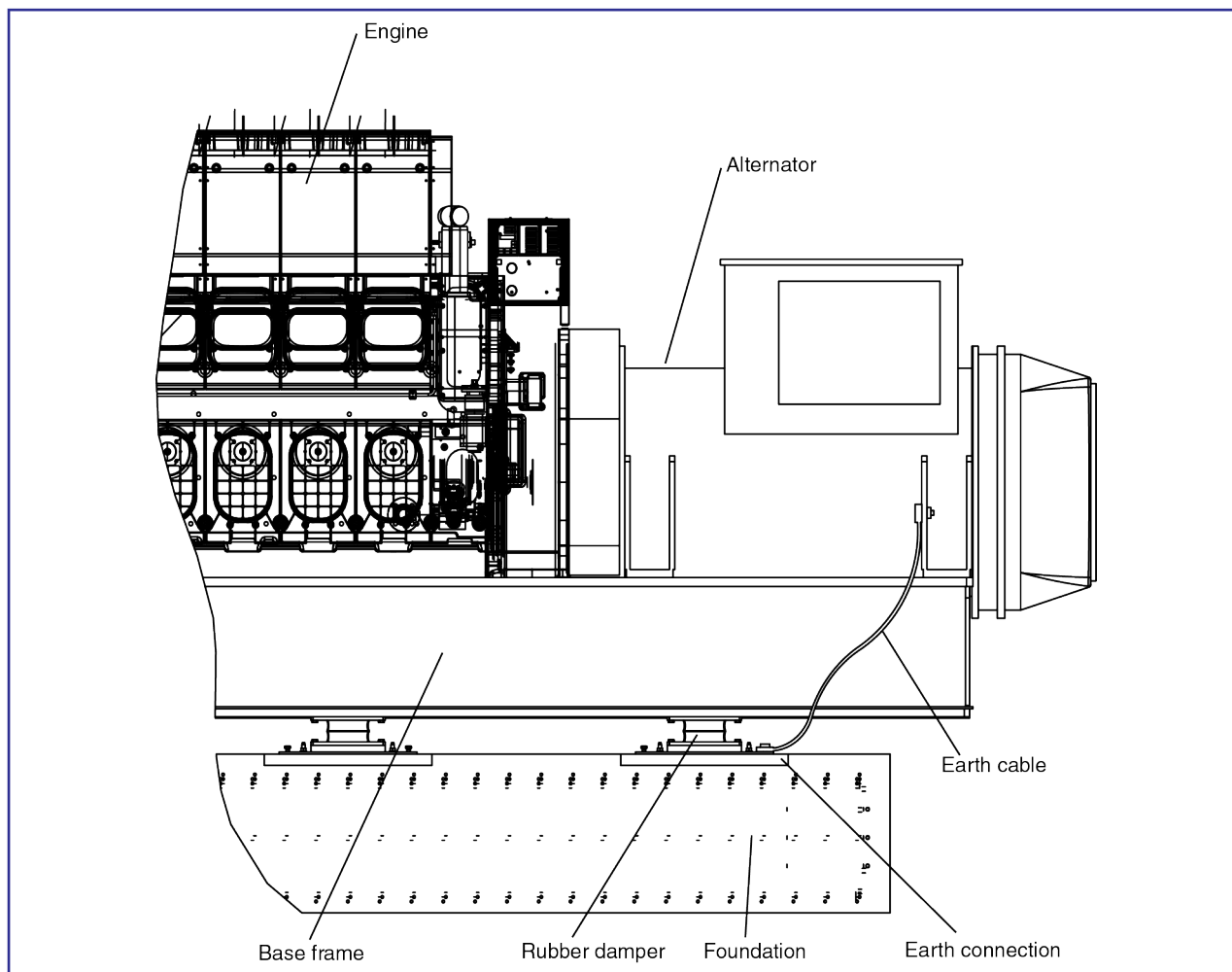
Figure 3: Stationary operation (example)
