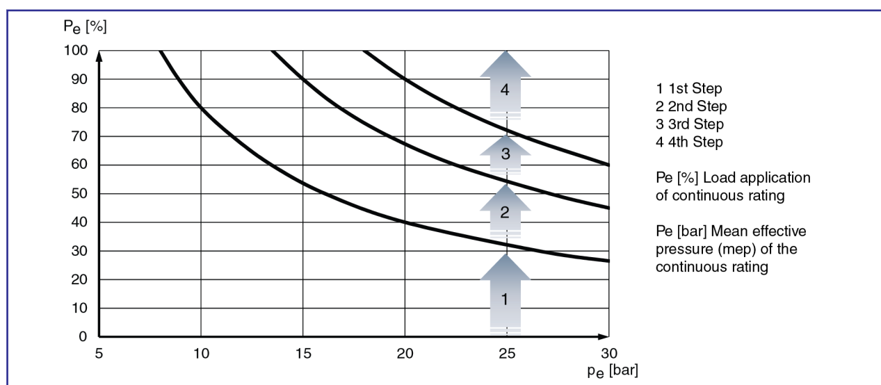
Fig. 1 Load application in steps as per IACS and ISO 8528-5.
