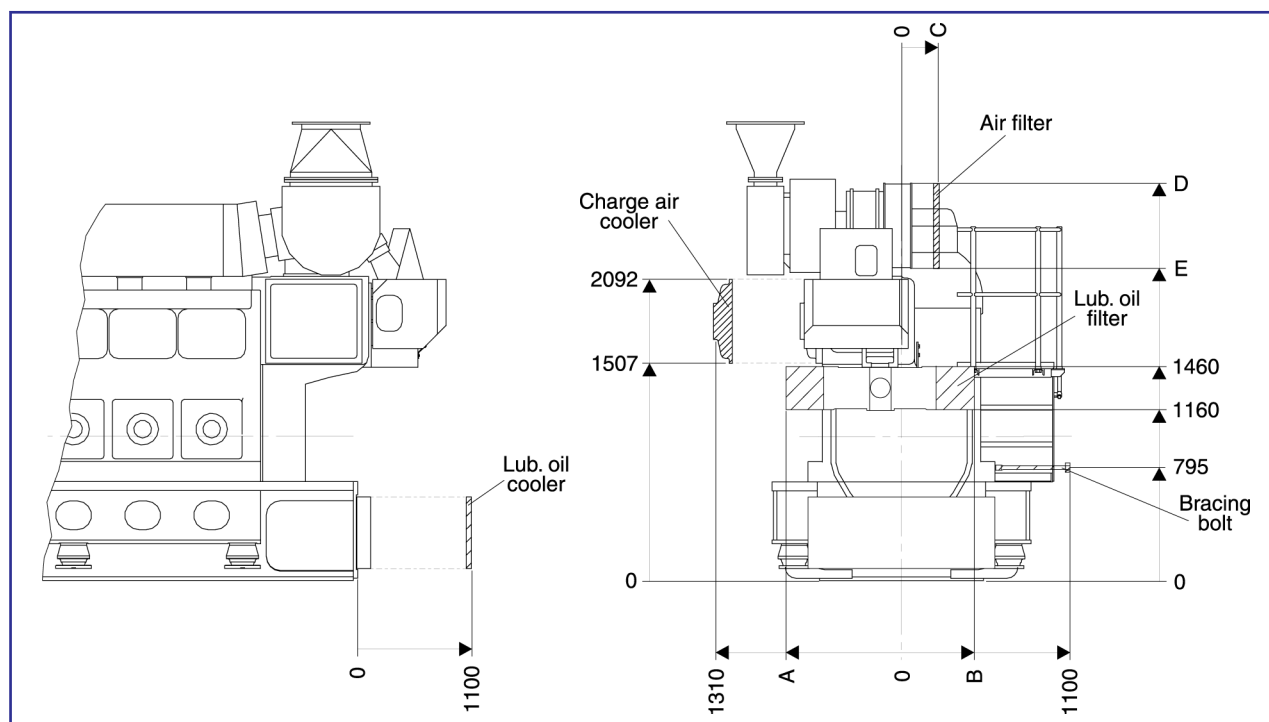
Figure 2: Overhaul areas for charge air cooler element, turbocharger filter element, lub. oil cooler, lub. oil filter cartridge and bracing bolt.
