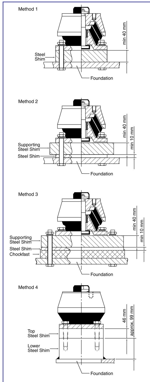
Figure 2: Support of conicals
