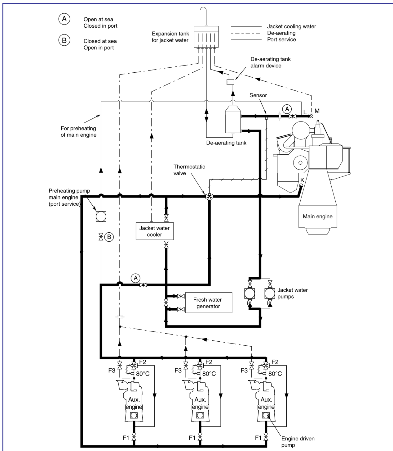
Figure 1: Operating at sea.
