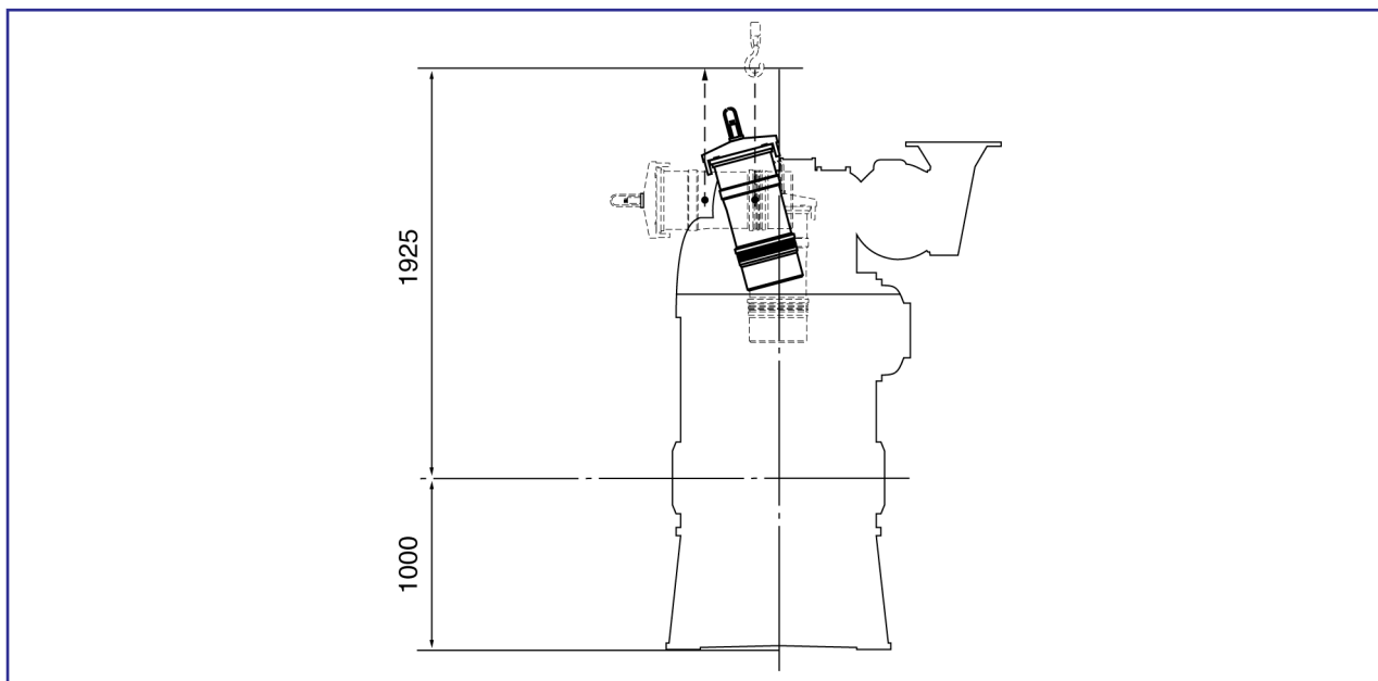
Figure 2: Minimum lifting height of cylinder liner only with special tools.
