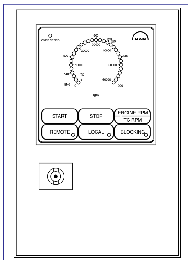
Figure 1: Starting box
