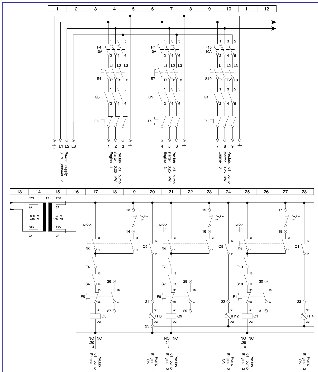
Figure 2: Wiring diagram.
