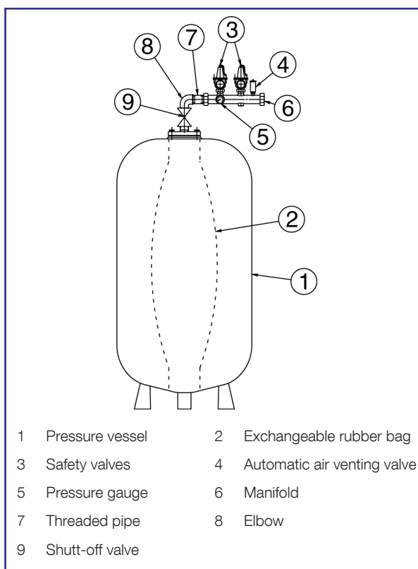
Figure 2: Expansion tank
