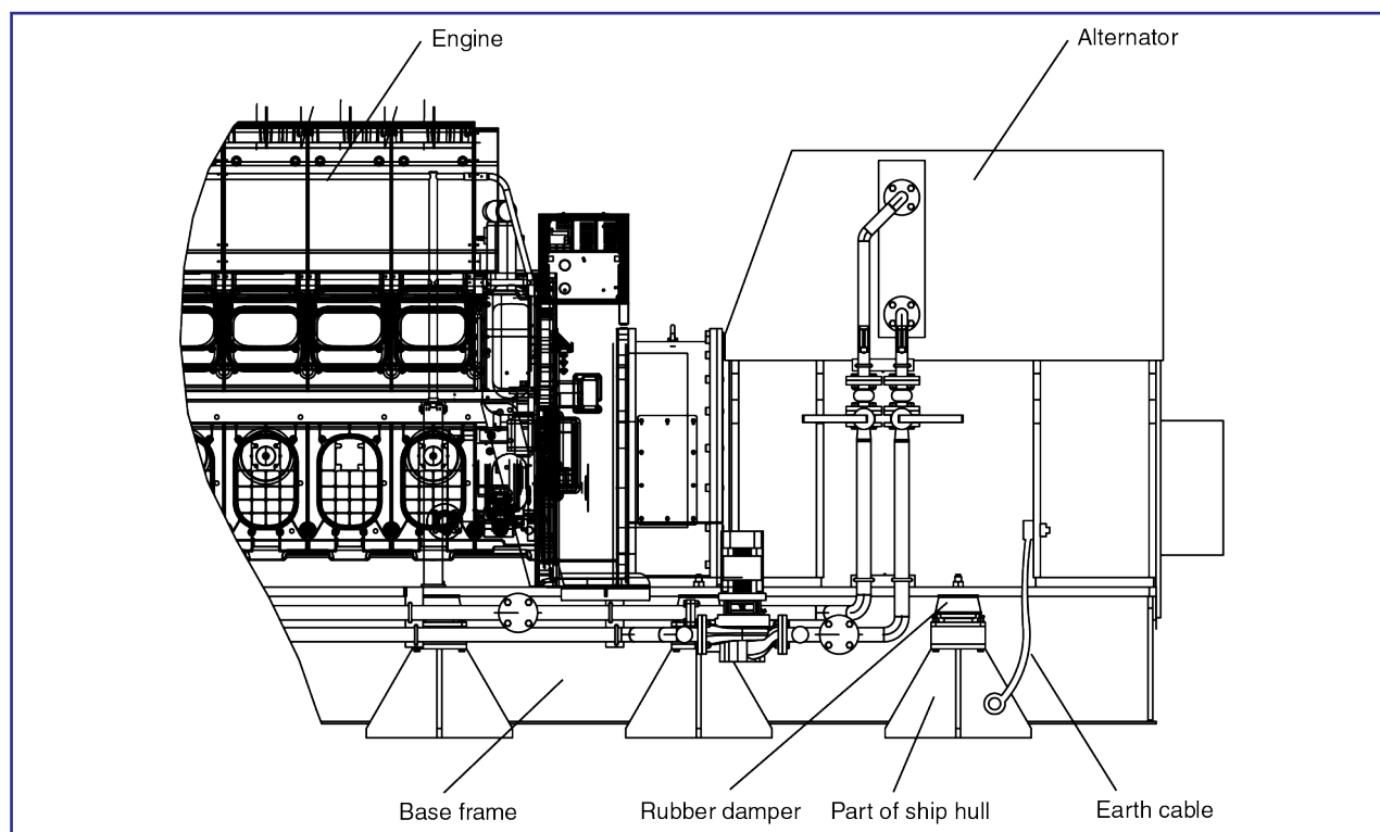
Figure 2: Marine operation (example)
