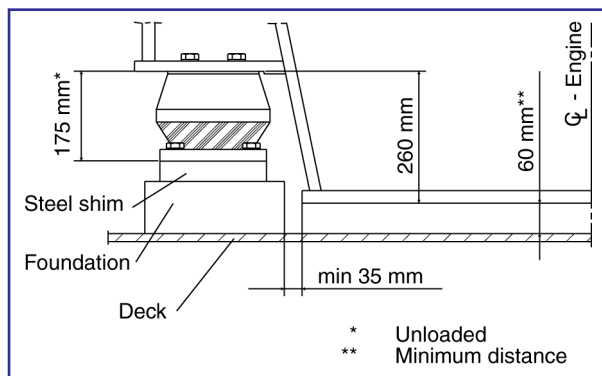
Figure 1: Resilient mounting of generating sets
