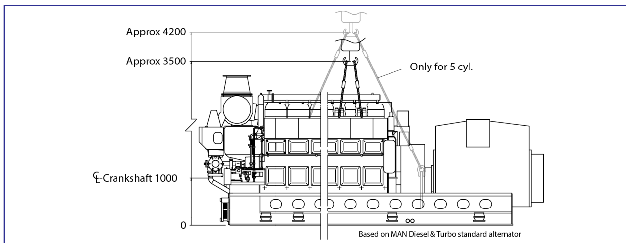
Figure 1: Crossbars' and wires placing on engine.
