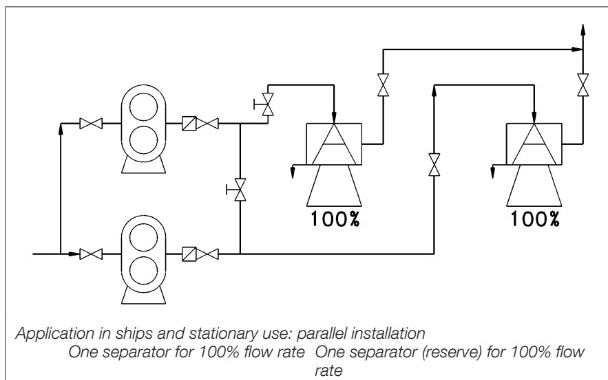
Figure 1: Arrangement of heavy fuel oil cleaning equipment and/or separator
