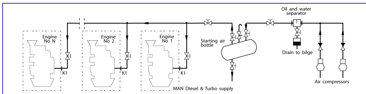
Figure 1: Diagram for compressed air system
