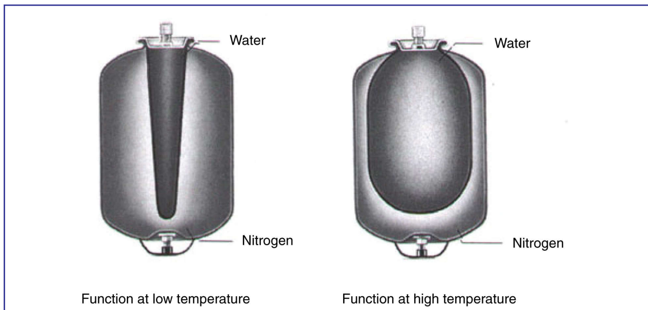
Figure 1: Function of expansion tank.
