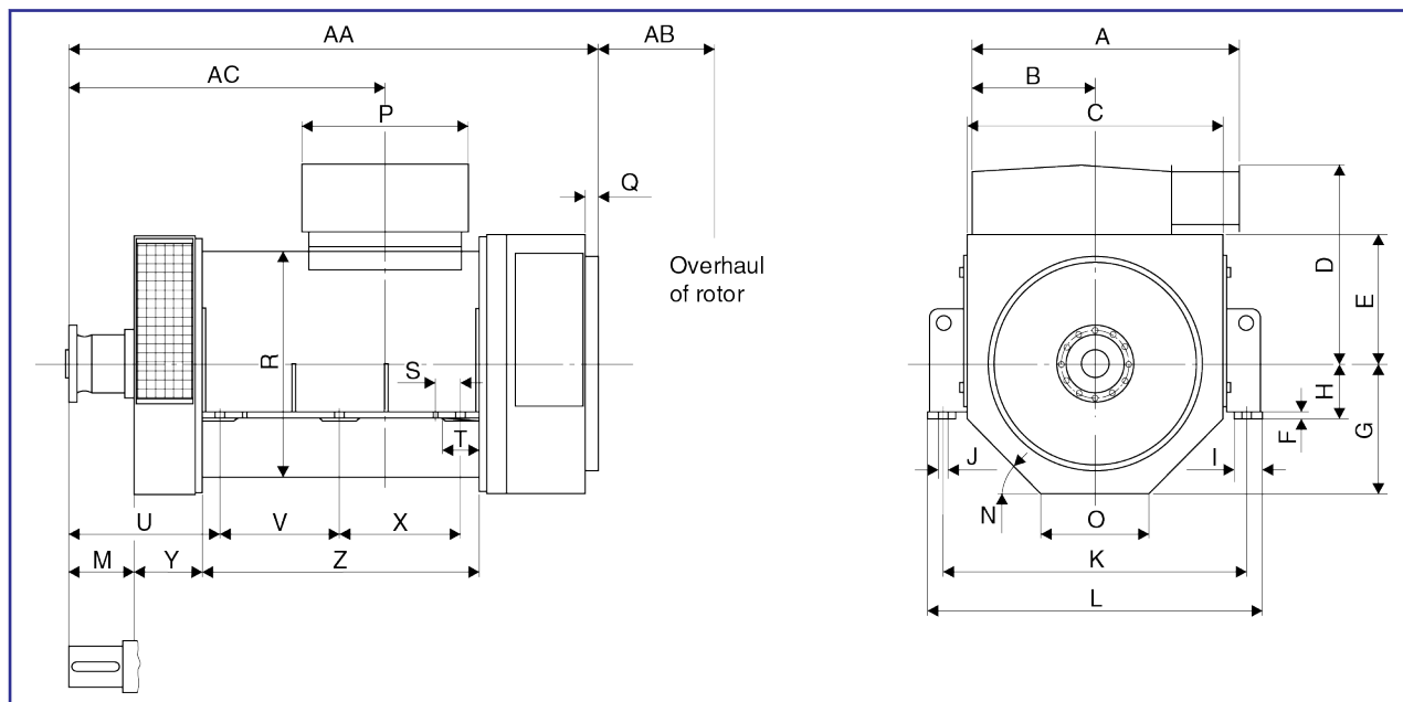
Figure 1: Outline drawing of alternator
