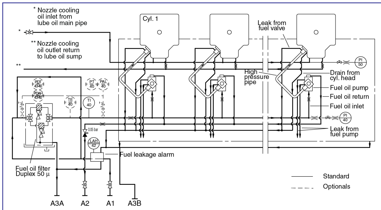
Figure 1: Diagram for fuel oil system (for guidance only, please see the plant specific engine diagram)
