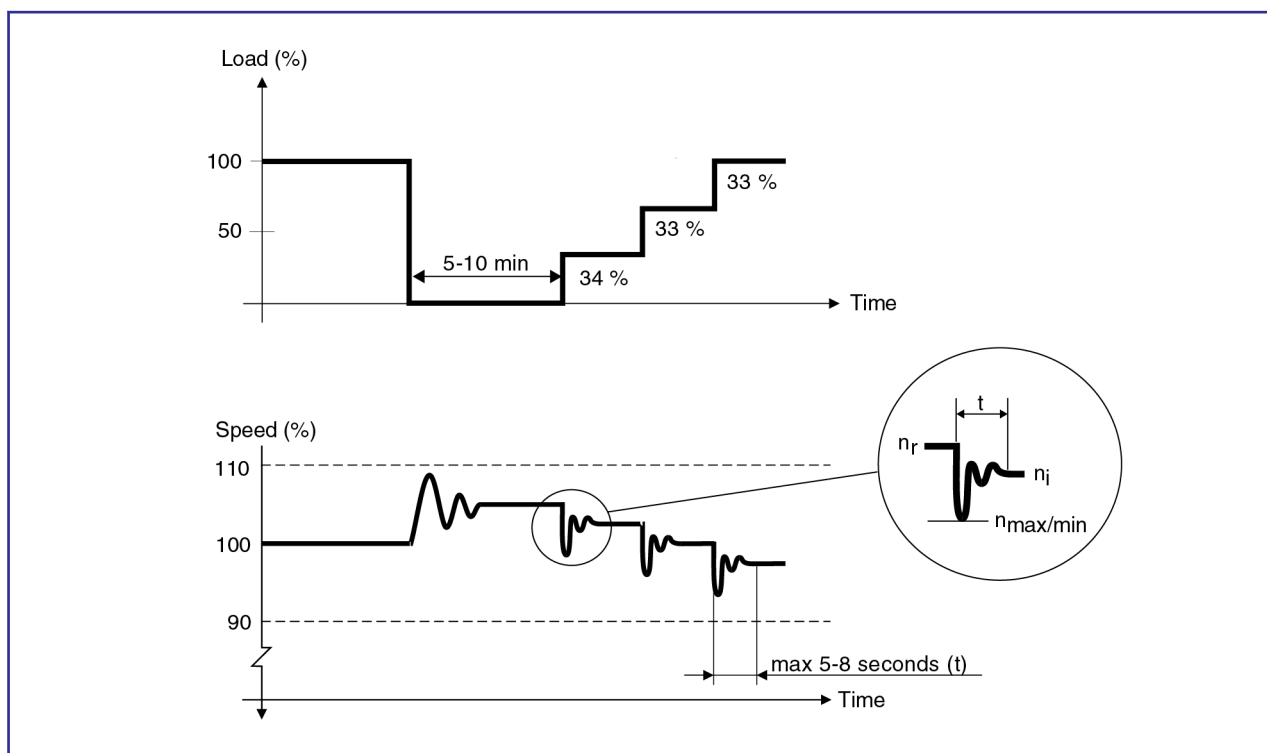
Fig. 4 Minimum requirements of the classification societies plus ISO rule.
