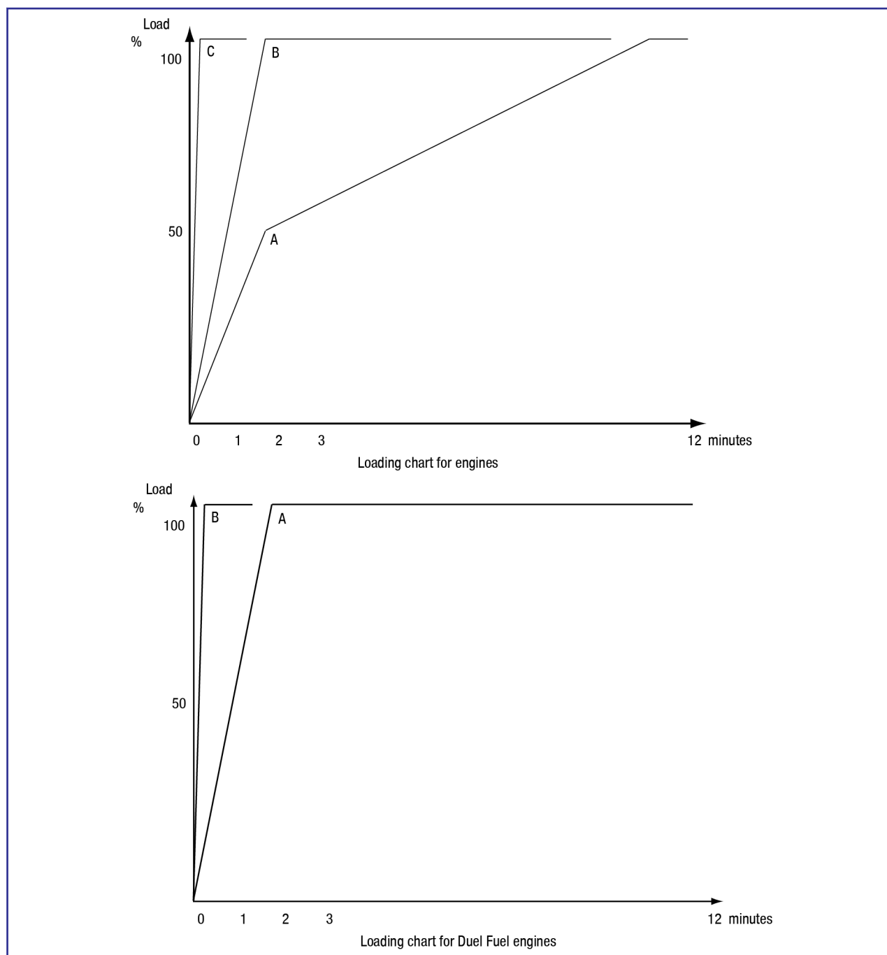
Figure 1: Loading chart
