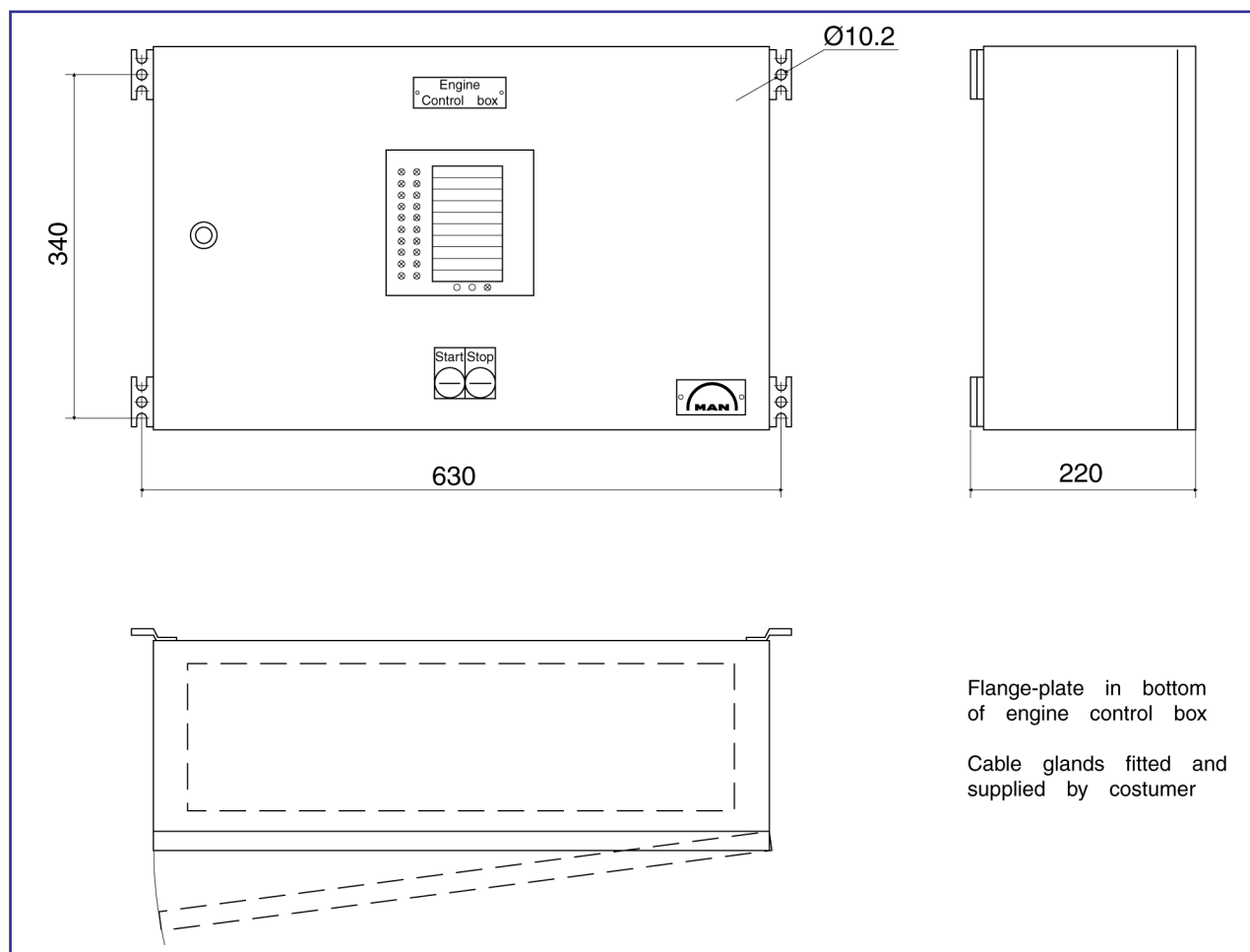
Figure 2: Engine control box.
