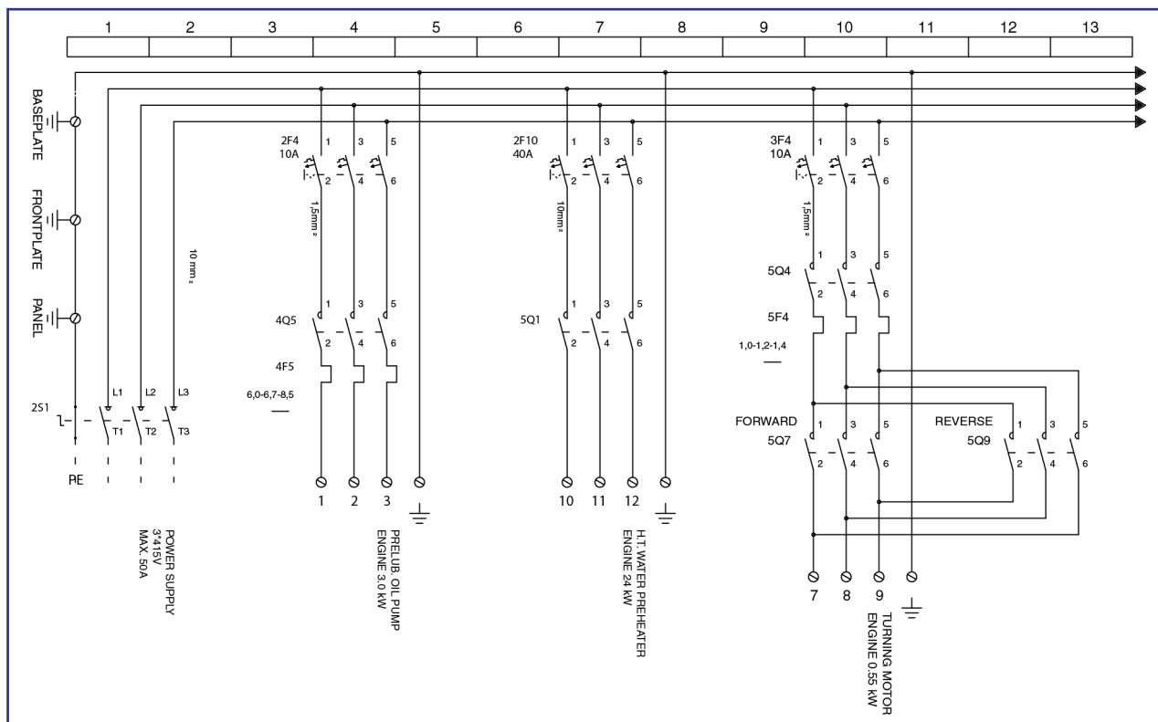
Figure 2: Wiring diagram
