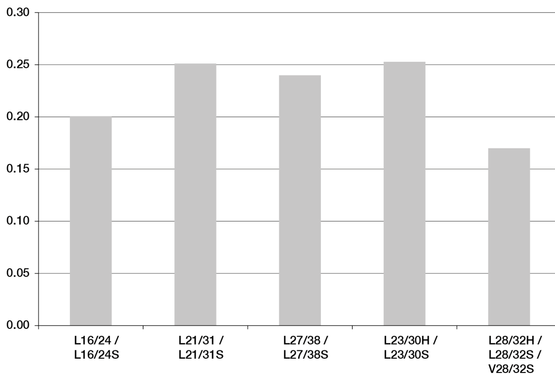
Figure 1: Leak oil on full load for MGO operation (for guidance only)
