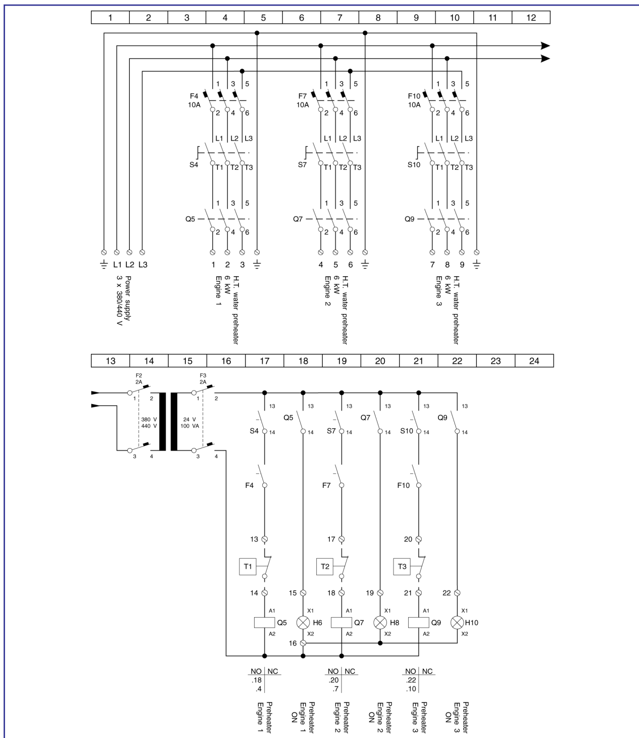
Figure 2: Wiring diagram.
