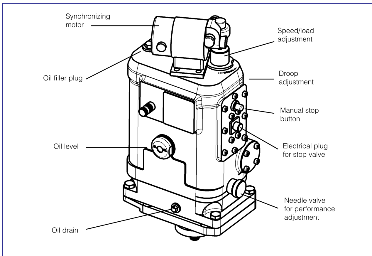
Figure 1: Regulateurs Europa governor.
