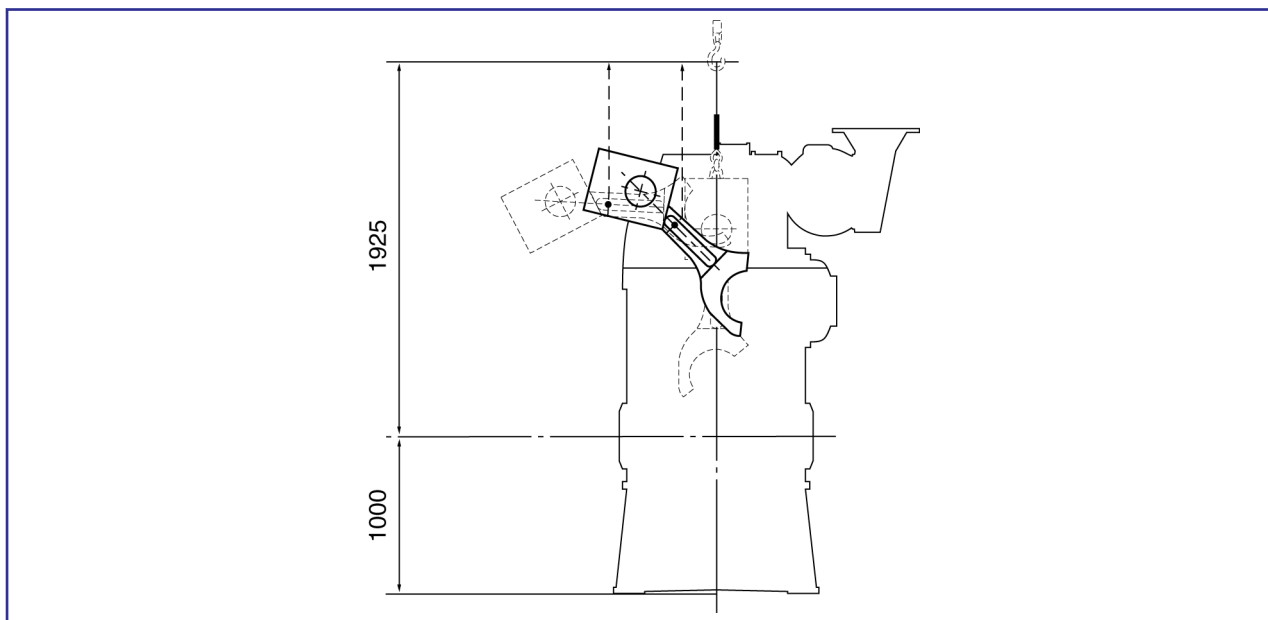
Figure 1: Minimum dismantling height of pistons only with special tools.
