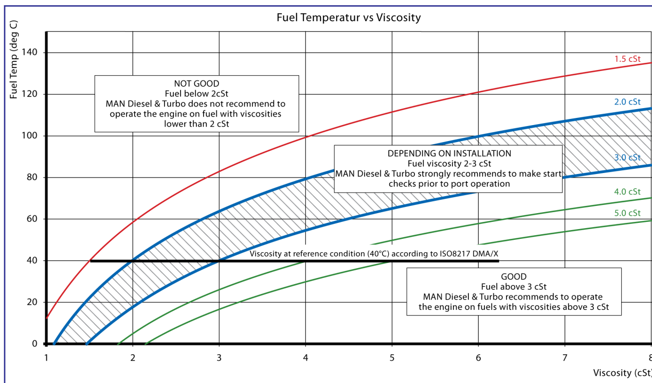
Figure 1: Fuel temperature versus viscosity.
