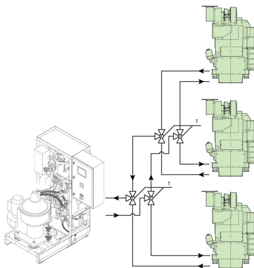
1 Interconnected valves
