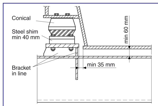
Figure 2: Transverse stiff deck structure.
