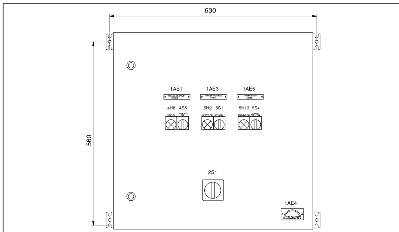
Figure 1: Dimensions
