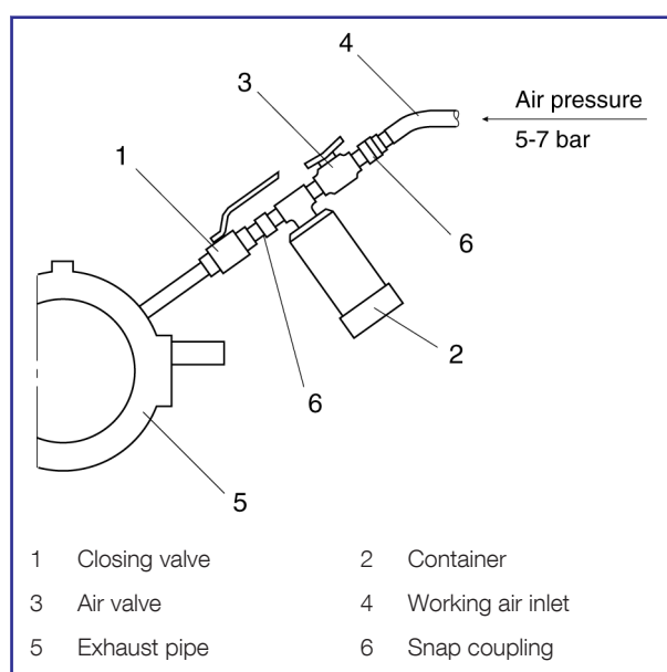
Figure 1: Arrangement of dry cleaning of turbocharger - turbine
