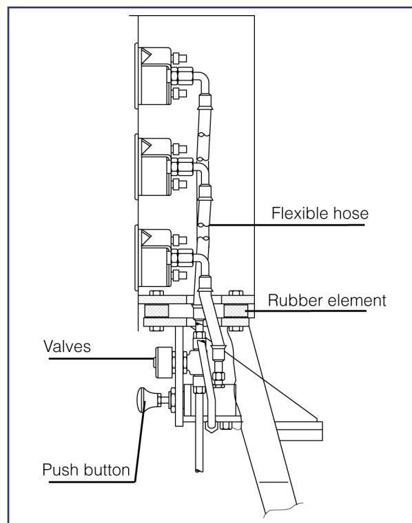
Figure 2: Cross section of instrument panel.
