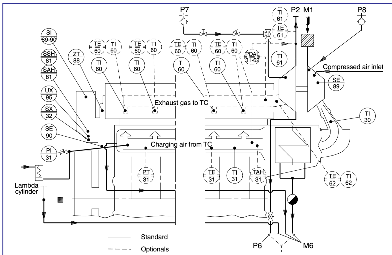
Figure 1: Diagram for combustion air system.
