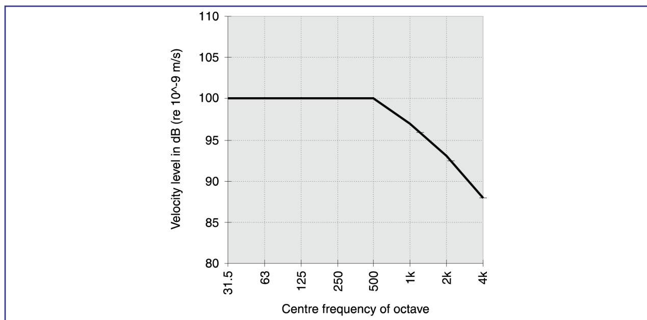
Figure 1: Structure-borne noise on resiliently mounted GenSets
