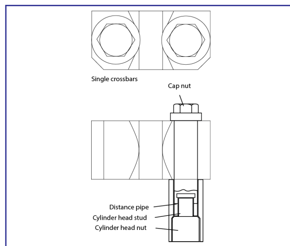
Figure 3: Crossbars.
