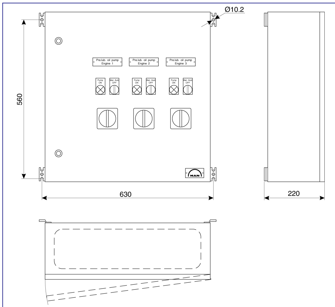
Figure 1: Dimensions.
