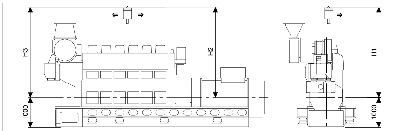
Figure 1: Dismantling height for piston
