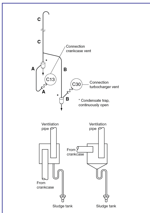
Figure 1: Crankcase ventilation
