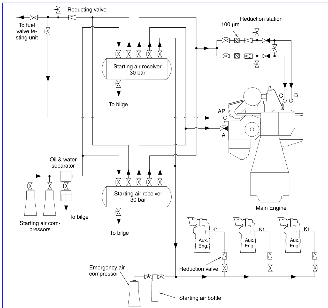
Figure 1: Starting air system
