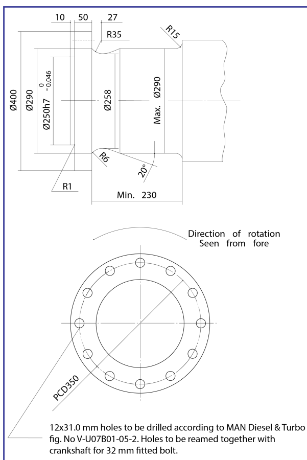
Figure 2: Shaft dimension for alternator, type B 16, cyl. 5 - 6 - 9
