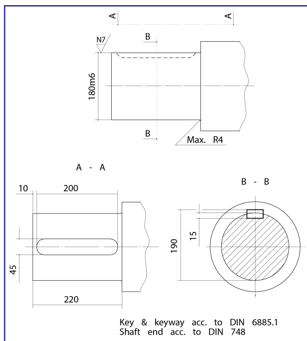
Figure 4: Shaft dimension for alternator, type B 20, cyl. 8
