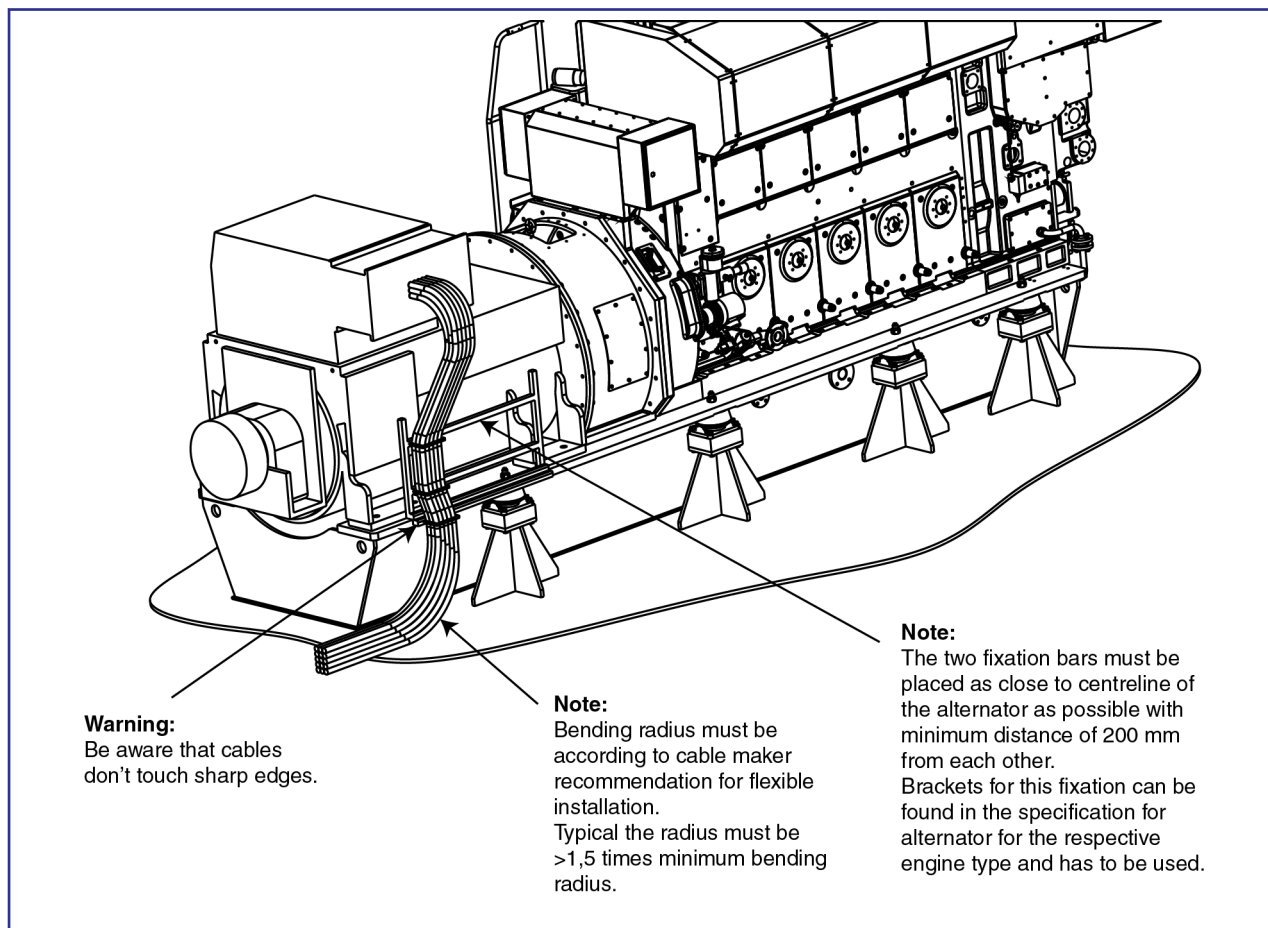
Figure 1: Connection of cables (example)
