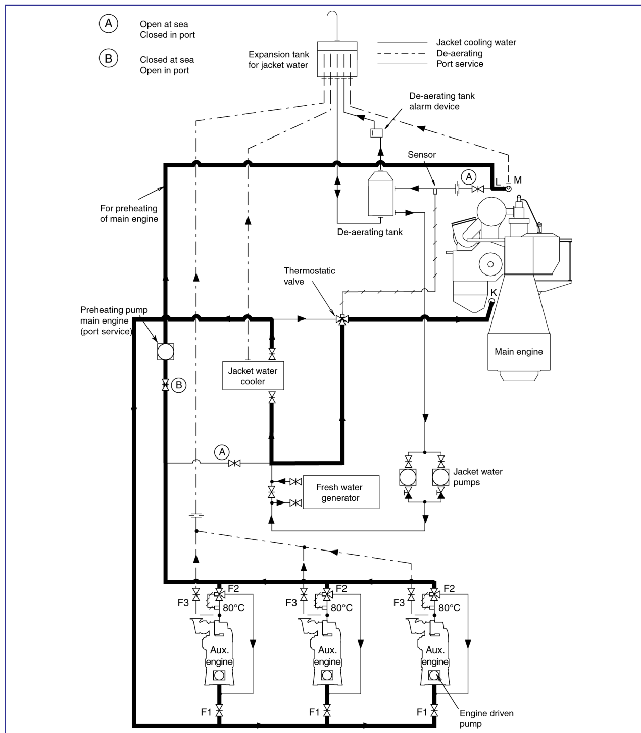
Figure 2: Operating in port.
