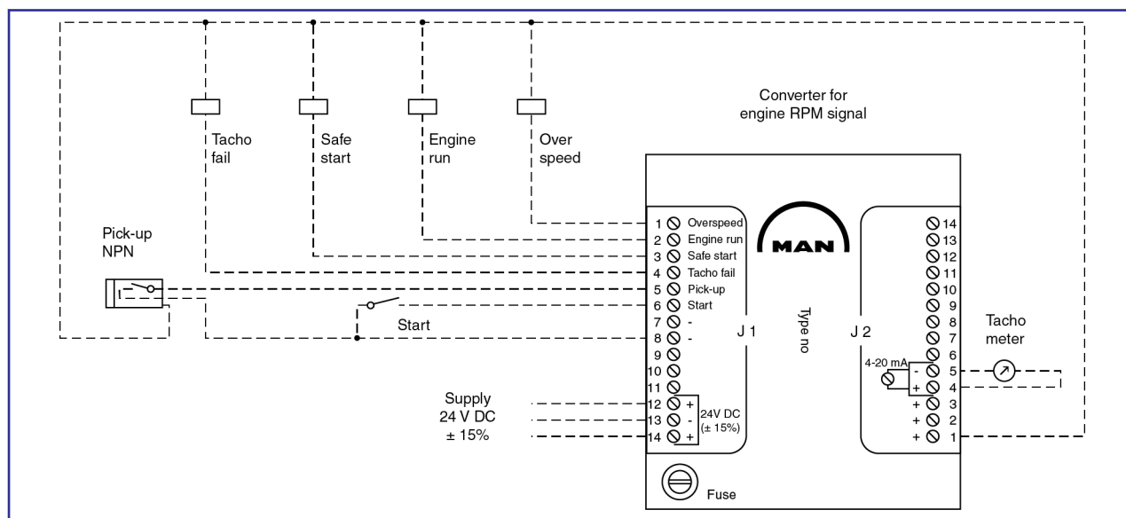
Figure 1: Converter for engine RPM
