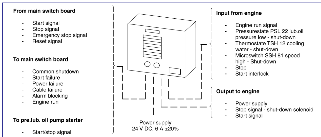
Figure 1: External connections to/from the engine control box.
