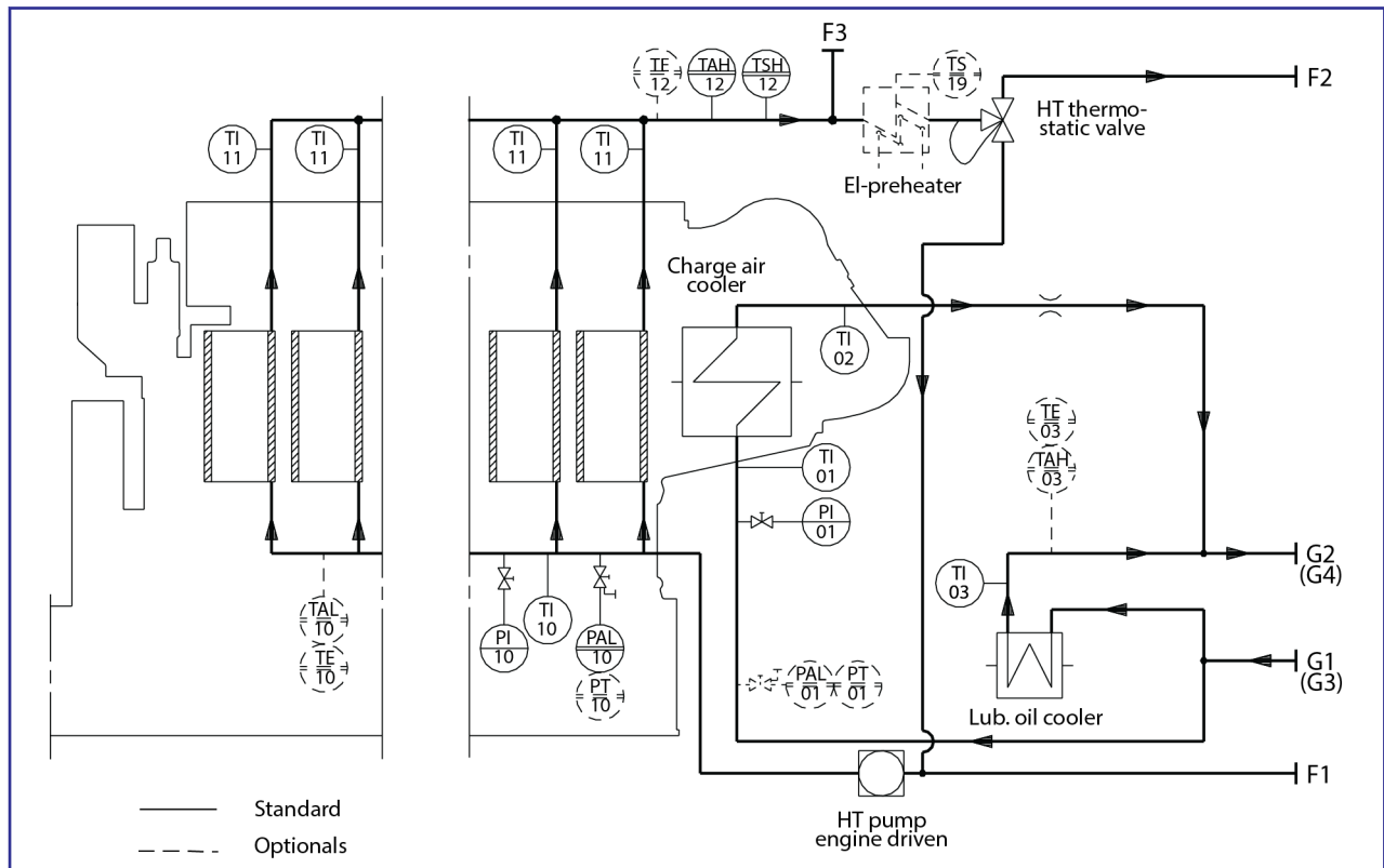
Figure 1: Diagram for internal cooling water system 2 (for guidance only, please see the plant specific engine diagram)
