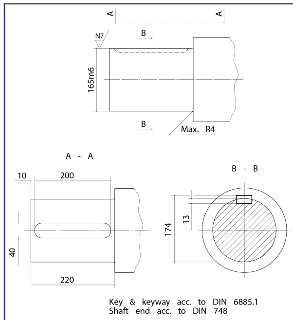
Figure 3: Shaft dimension for alternator, type B 20, cyl. 7
