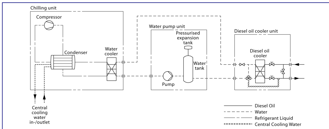
Figure 2: Chiller.
