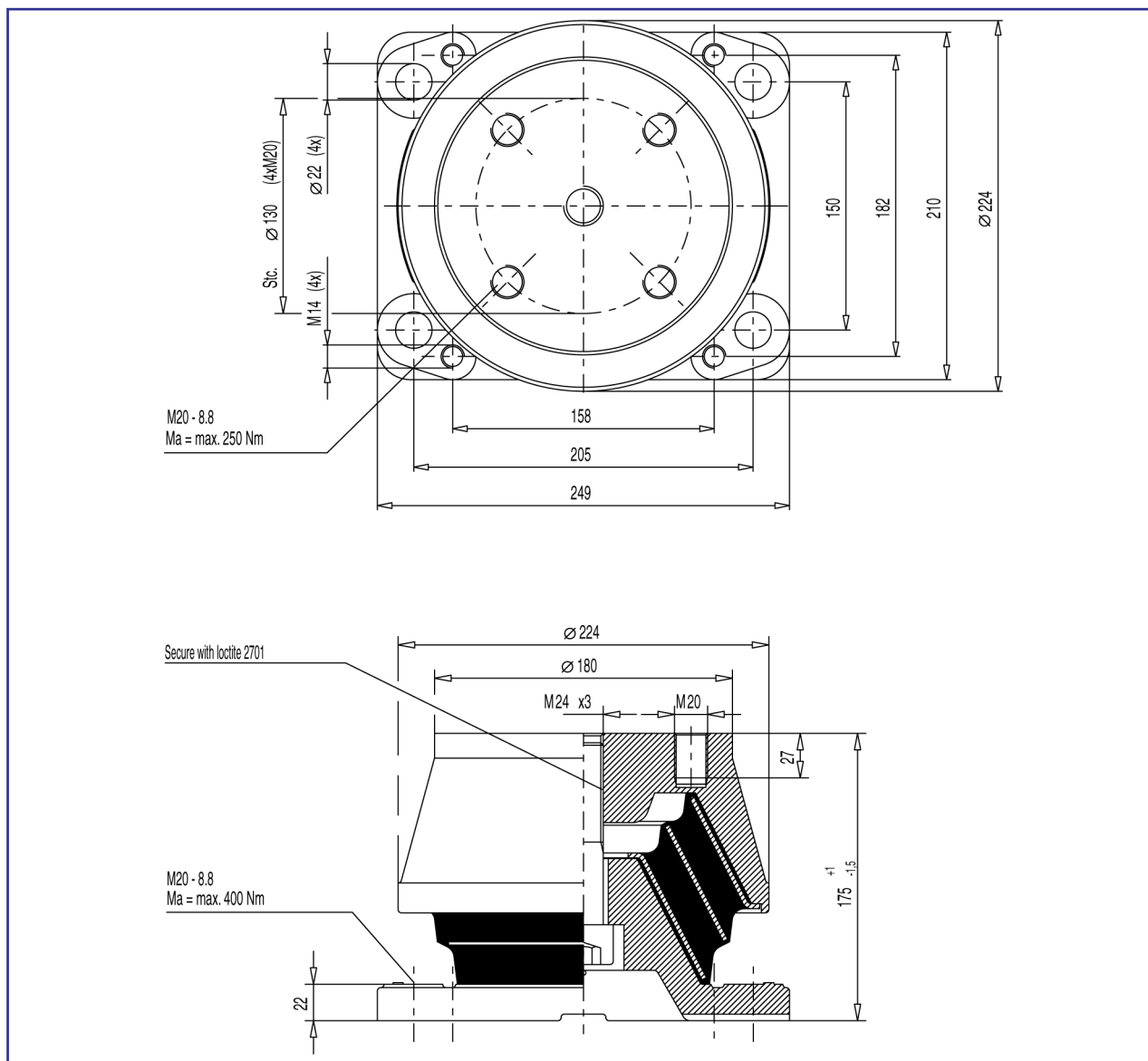
Figure 3: Conical mountings
