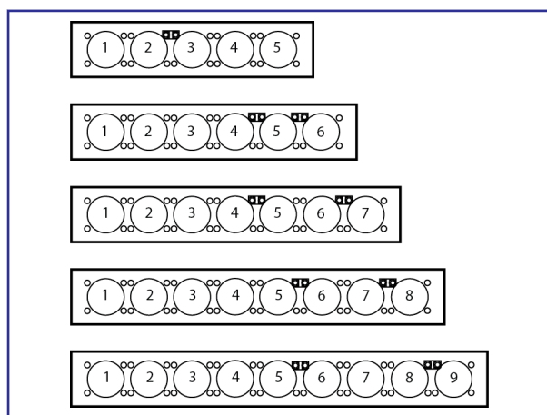
Figure 2: Crossbars' placing on engine.
