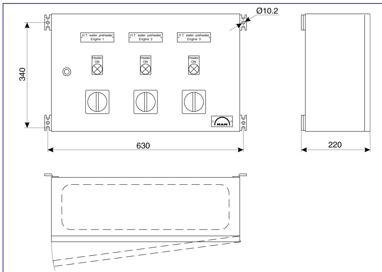
Figure 1: Dimensions of the control cabinet.
