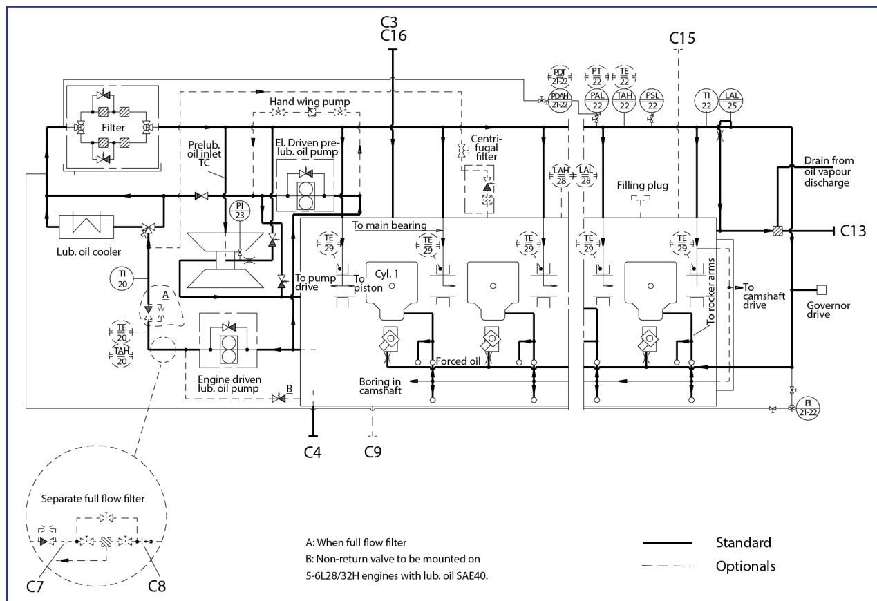
Figure 1: Diagram for internal lubricating oil system (for guidance only, please see the plant specific engine diagram).
