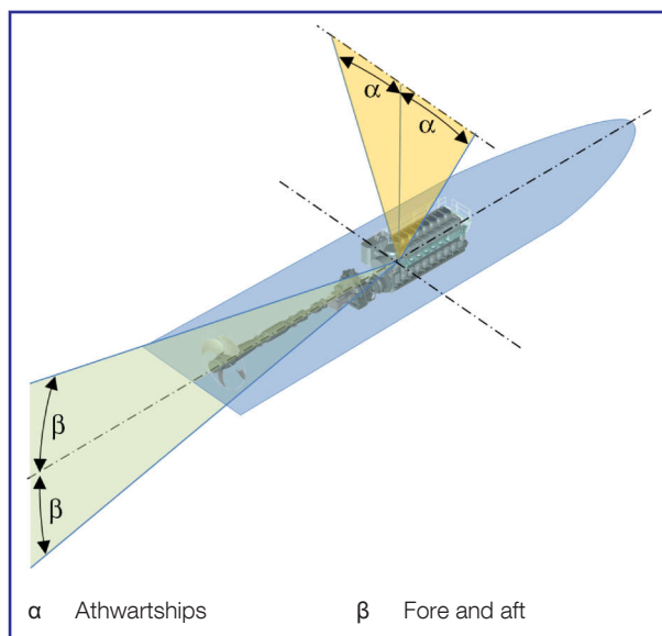
Figure 1: Angle of inclination.
